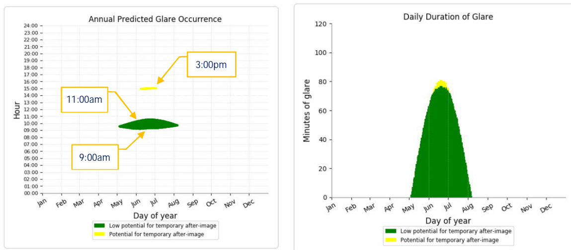
Figure 16 Selected SGHAT Results: FIXED TILT 15° WEST Mode (Runway 29)
