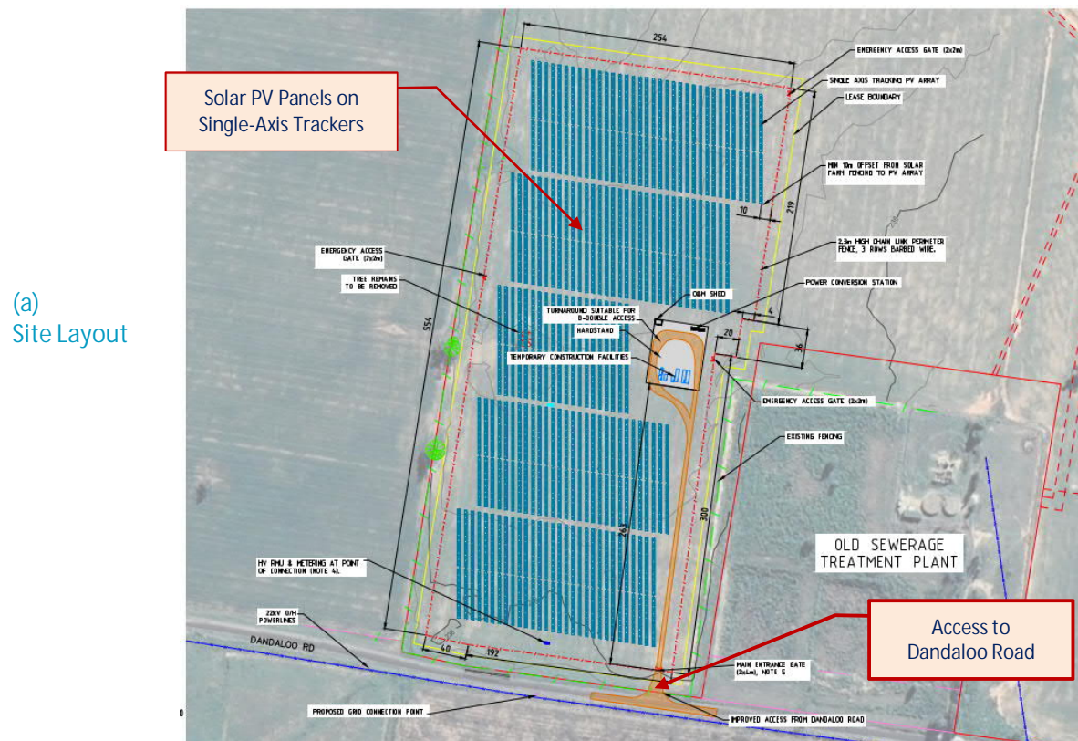
Figure 2 Narromine West Solar Farm Site Layout
