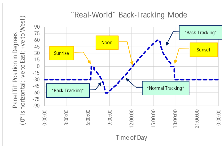
Figure 13 Example 24-Hour "Back-Tracking" Operational Mode (around equinox)
