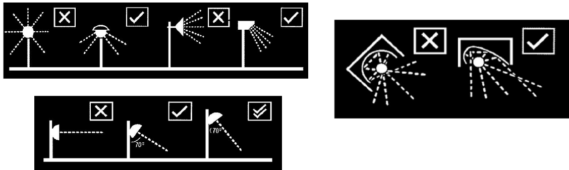
Figure 22 Luminaire Design Features that Minimise Light Spill
